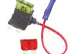
ATC fuse; main fuse at specified circuit rating up to 40A max. Added circuit up to 10A max.
